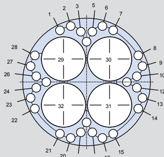
Contact Arrangement 21-200
