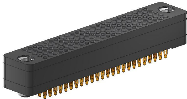
GSTB-120-.095-G1 Bottom Mounted Connector
