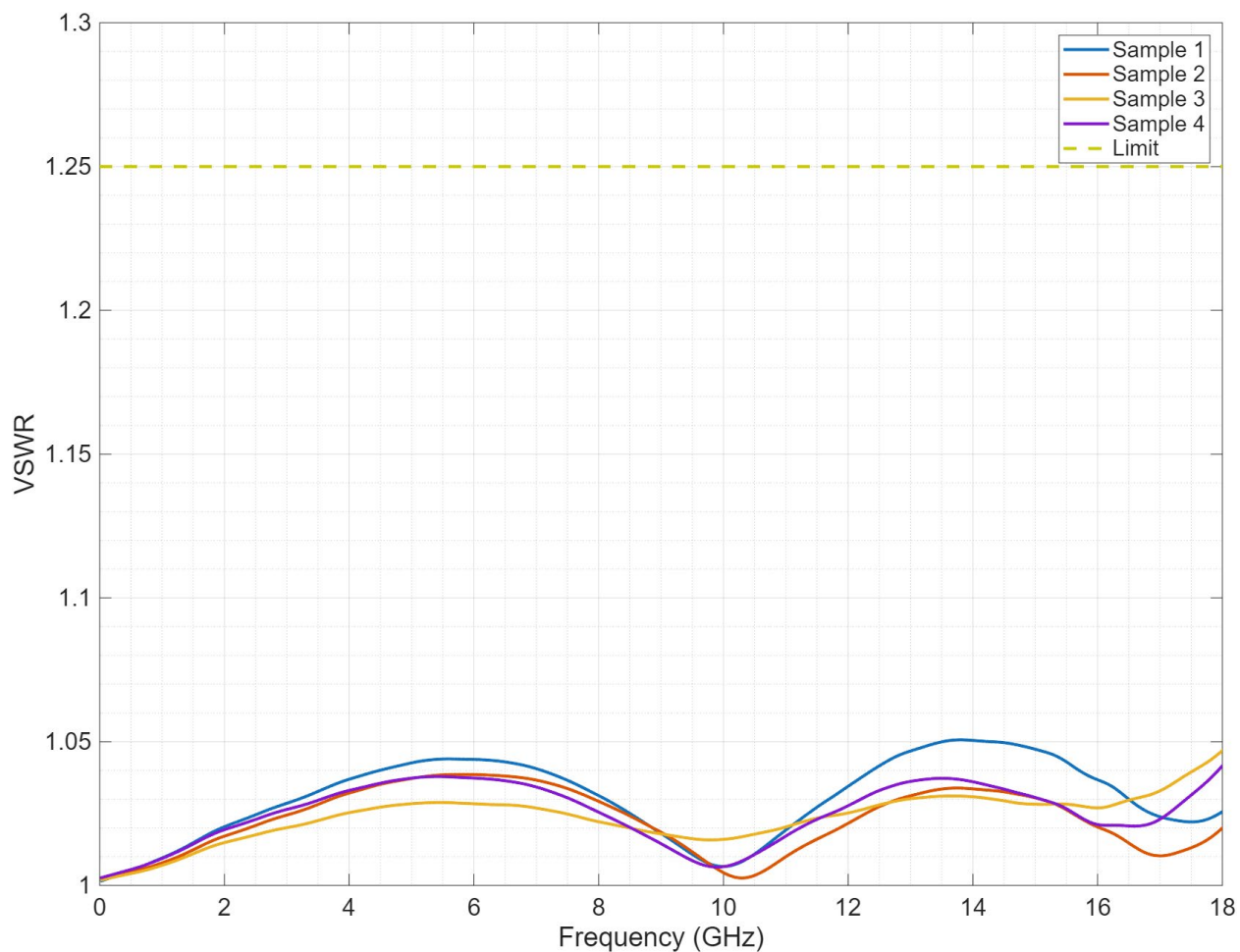
Figure 3. Connector VSWR
