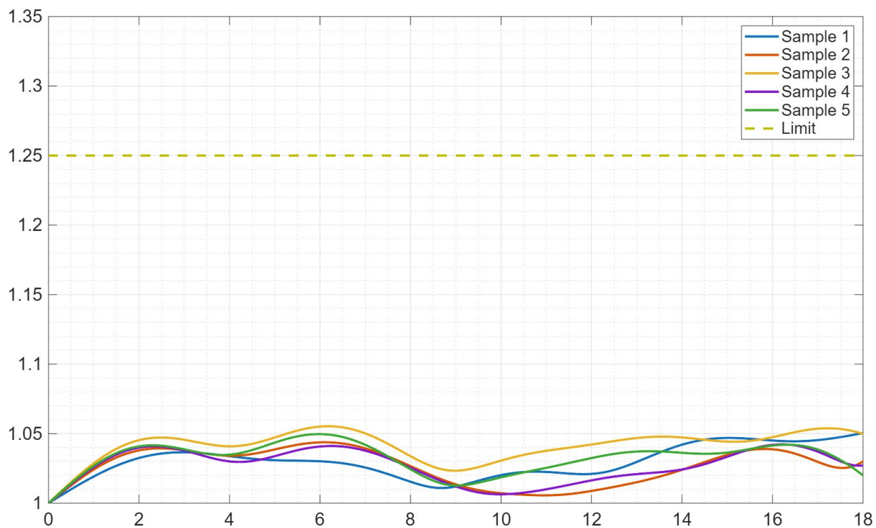
Figure 3. Connector VSWR
