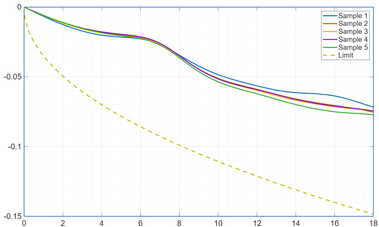
Figure 2. Connector Insertion Loss
