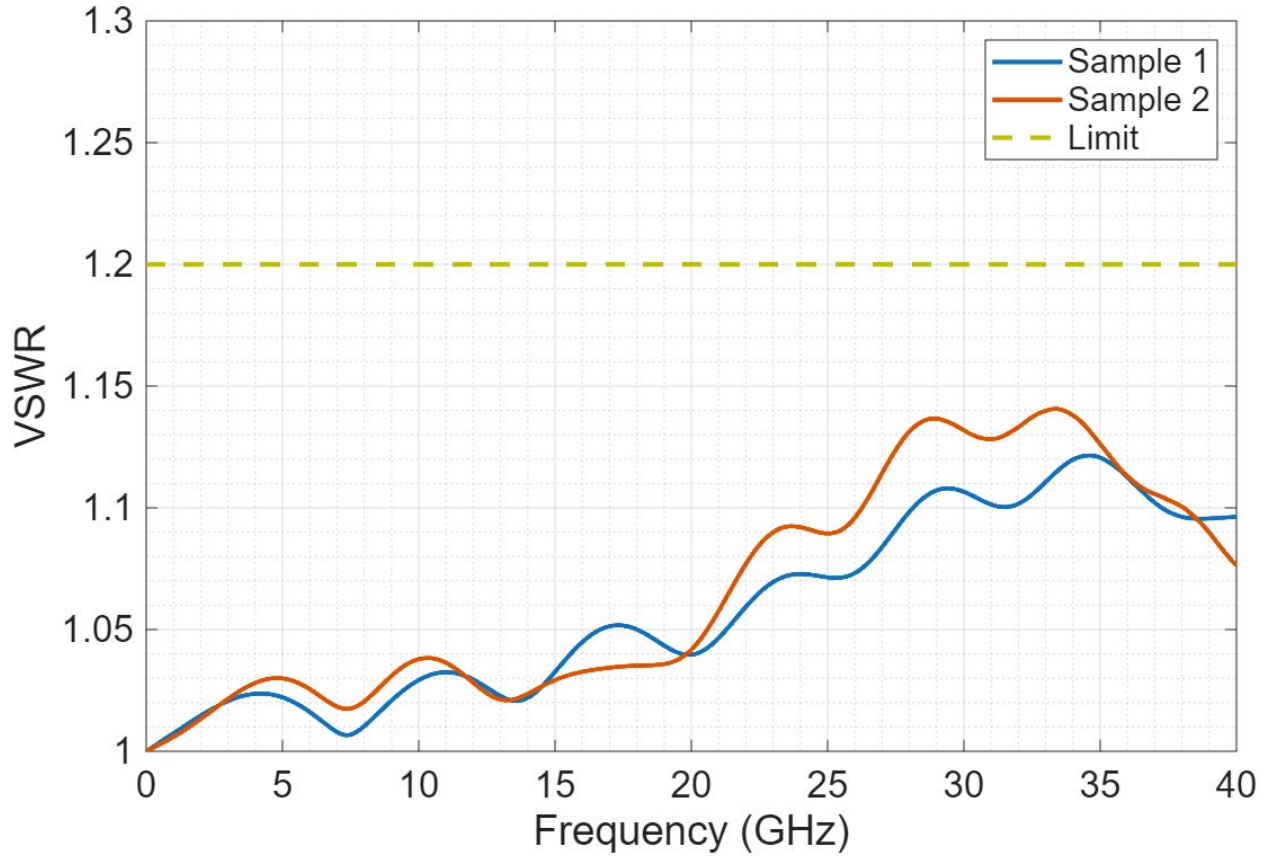
Figure 3. Connector VSWR
