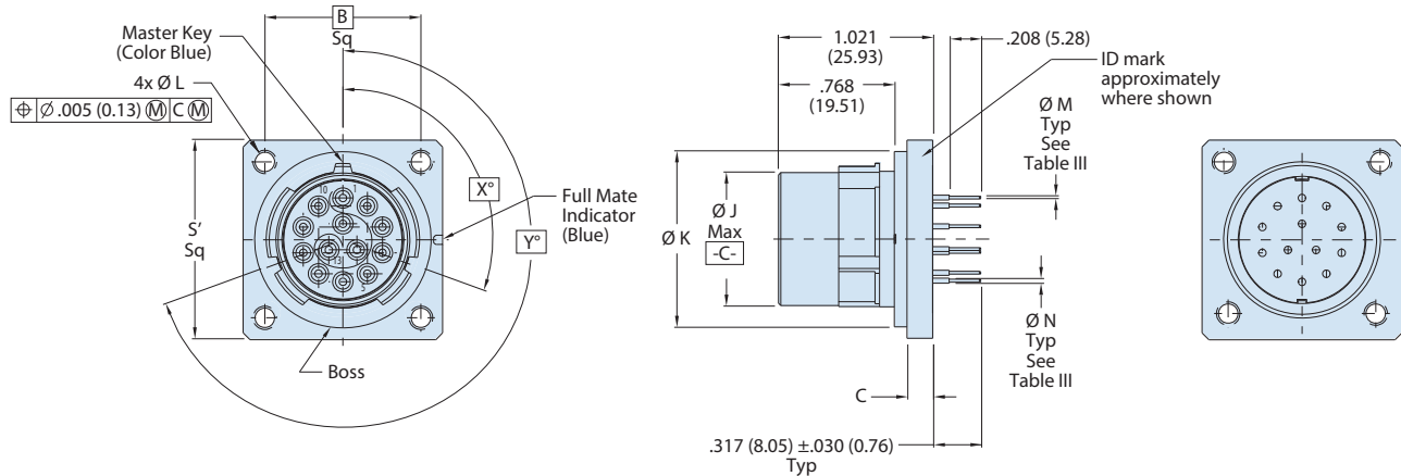
HS WALL MOUNT STANDARD HELICOIL
