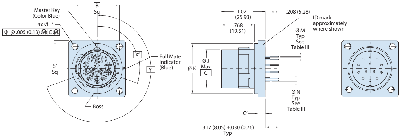
HM WALL MOUNT METRIC HELICOIL
