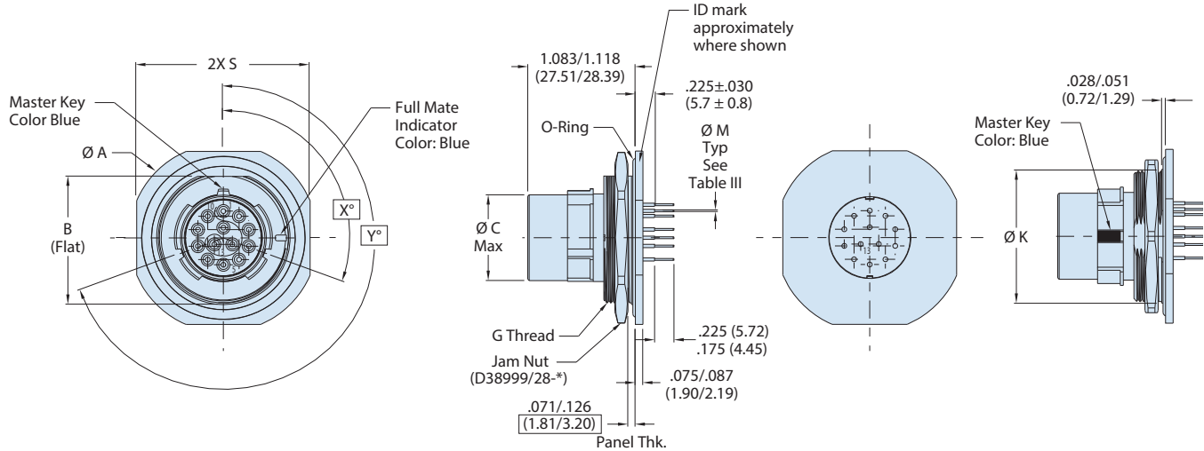
Jam-Nut Receptacle (REF: MIL-DTL-38999/44)
