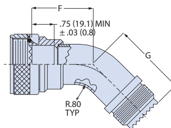
Profile M 45°
