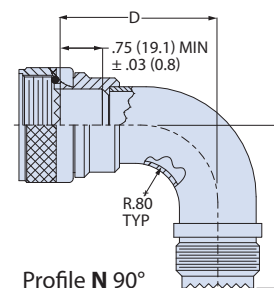
Profile N 90°
