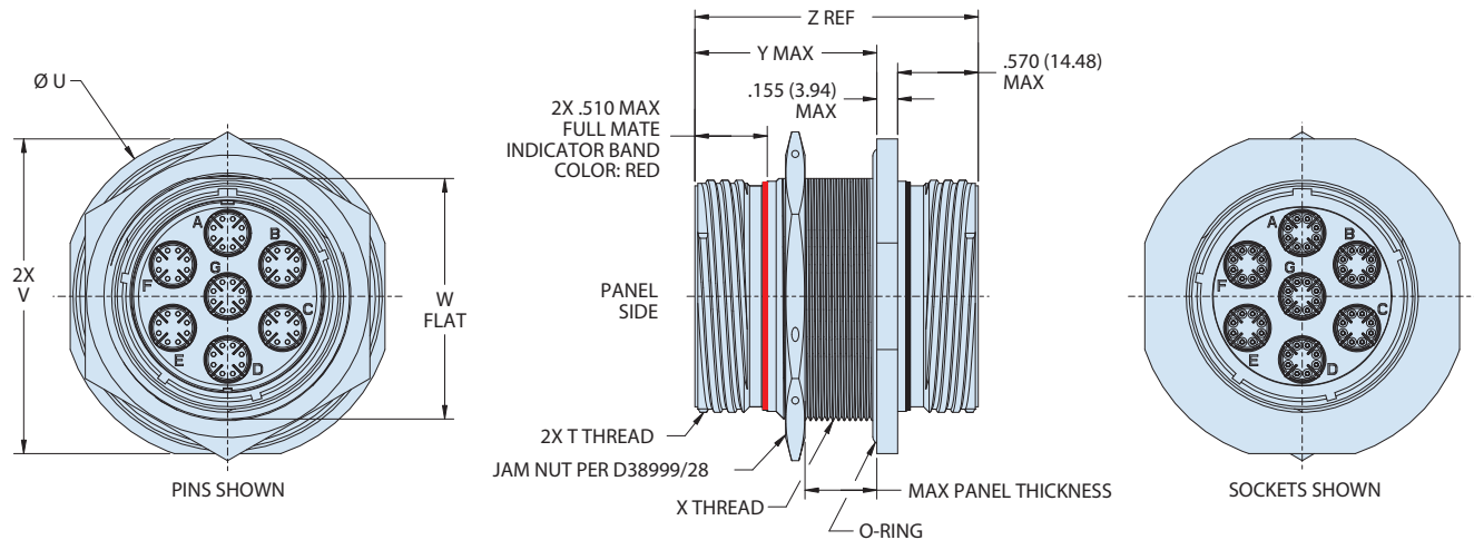
Jam-Nut Dimensions
