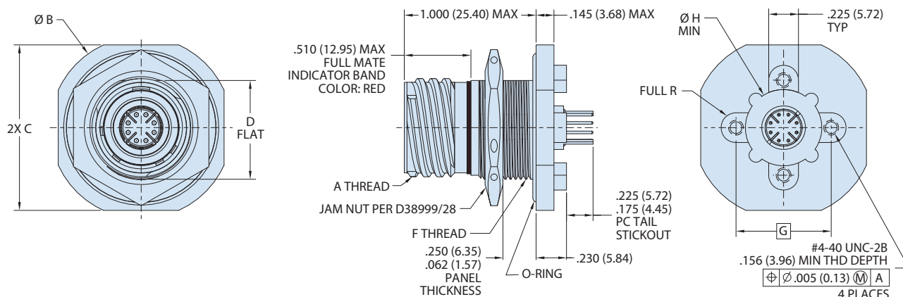
Jam-Nut Mount Dimensions
