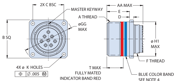
DO & DD0- WALL MOUNT RECEPTACLE WITH STANDARD HOLES DIMENSIONS
