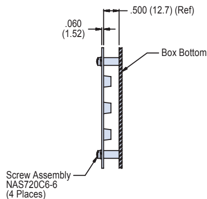
VIEW C-C
