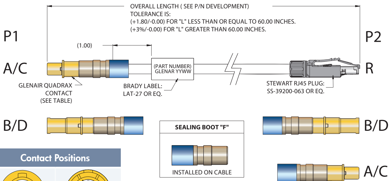
Quadrax contact, Pin and Socket
