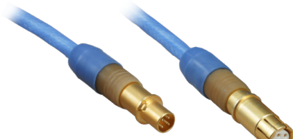
Quadrax contact, Pin and Socket
