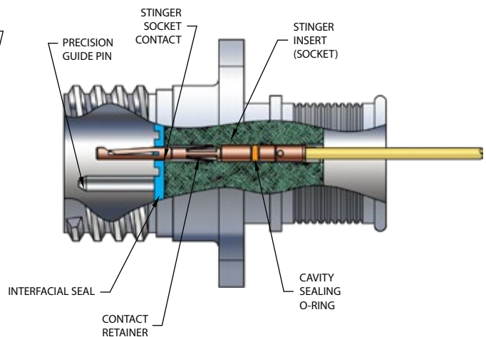
Receptacle Cross-Section (841 shown)
