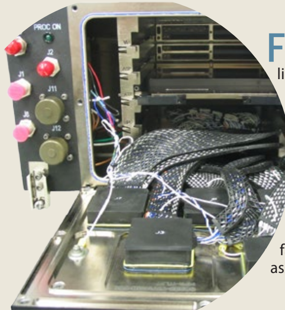
Non-environmental aircraft cable with integrated circuit breakout box and Mighty Mouse 804 push-pull connectors
