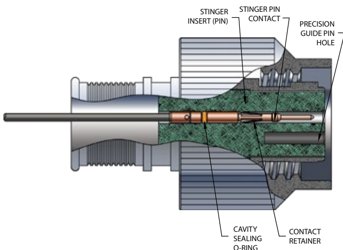
Plug Cross-Section (841 shown)
