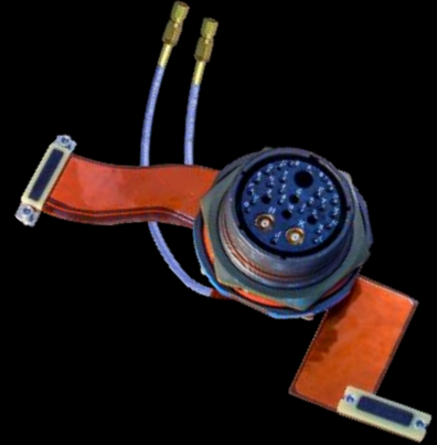
Turnkey Coax interconnect assemblies
