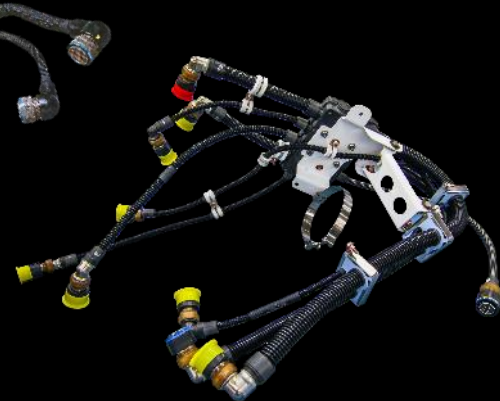
Factory-terminated conduit assemblies
