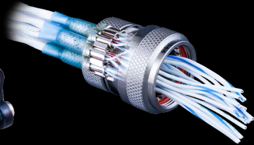
StarShield zero-length shield termination
