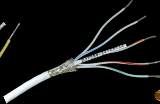
M27500 type and custom multi-conductor cables
