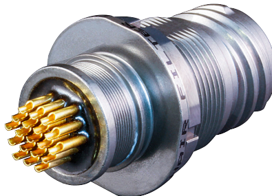
Series 80 Mighty Mouse solder-cup filter receptacle with integrated banding porch
