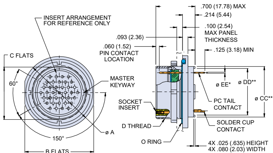
Jam-Nut Dimensions
