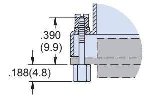
Hex Socket Jackscrew
