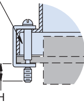
Code F Female Jackpost
