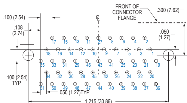
51 SOCKET M83513/14-G
