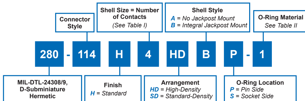
SHELL STYLE "A" O-RING LOCATION "S"
