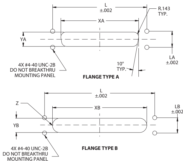
RECOMMENDED PANEL CUTOUT SEE TABLE II
