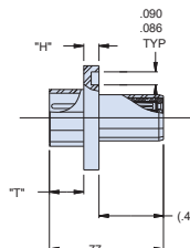
SHELL STYLE "B" O-RING LOCATION "P"
