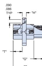
SHELL STYLE "B" O-RING LOCATION "P"
