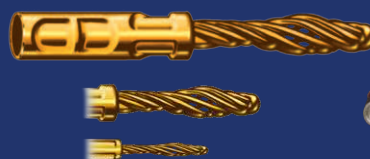
Low-resistance TwistPin contacts: micro, nano, D-sub, crimp, and factory-terminated
