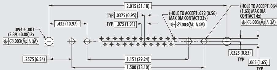
Contact numbers are mating face of pin connector. Socket connector contact numbers are reversed.
