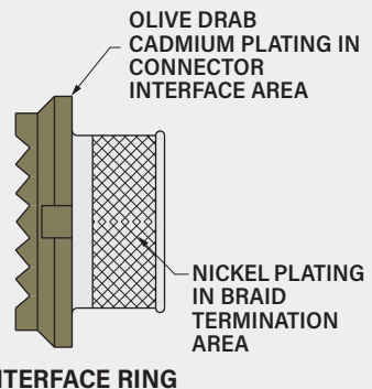
INTERFACE RING
