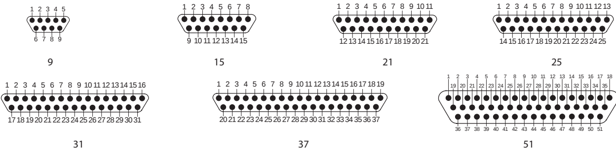
Mating face of pin connector. Socket connector contact numbers are reversed.
