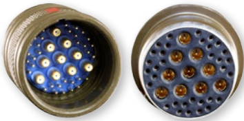
QDC Quick-Disconnect Push-Pull Mating
