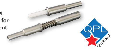
Glenair optical fiber test probes and connector adapters provide accurate and repeatable testing of MIL-DTL-38999 F/O assemblies
