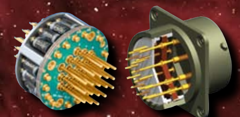
Planar Array EMI/EMP Filter Connectors
