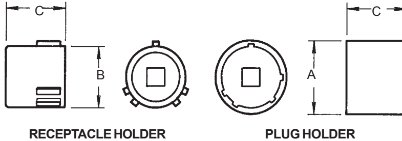
RECEPTACLE HOLDER
