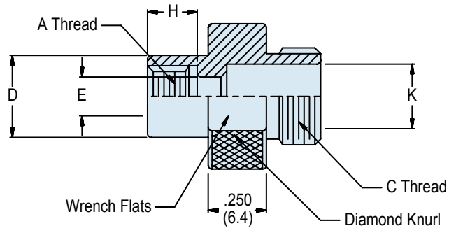
Optional Configuration Supplied when E Diameter is Equal or Less than K Diameter
