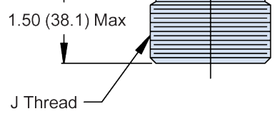
TYPE A - Plug Cap For use with MS17344
