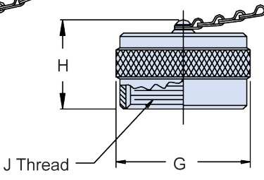
TYPE B - Receptacle Cap For use with MS17343, MS17345, and MS17347
