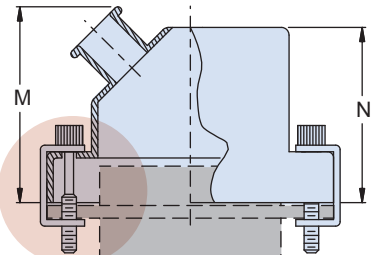
Code H Extended Jackscrew
