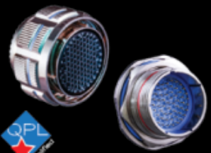
MIL-DTL-38999 Series III environmental connectors
