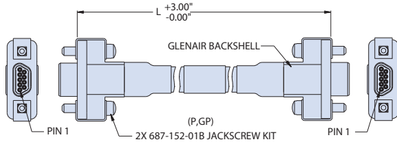
BACK TO BACK WIRING CABLE ASSY TYPE -A ECSS-E-ST-50-12C REV 1, FIGURE 5-4
