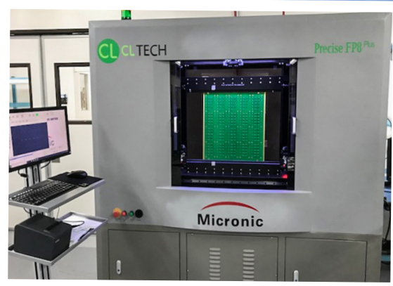
Automated Optical Inspection and Flying Probe Electrical Test
