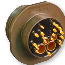
MIL-STD-1760 filtered umbilical connector
