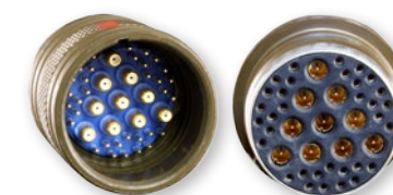
QDC Quick-Disconnect Push-Pull Mating
