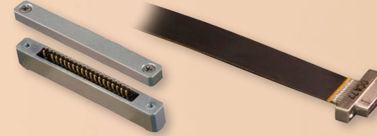
AlphaLink® Board-Level Connectors and Flex Jumpers
