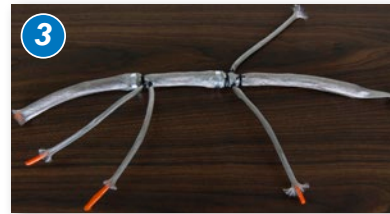
Choose user-installable microfilament tubular braid in twelve standard diameters. Assemble per standard multi-branch cable shielding processes, as above.
