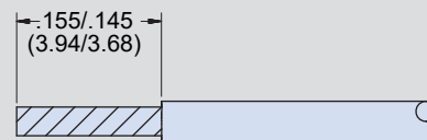
RECOMMENDED WIRE STRIP LENGTH
