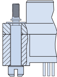
S Style Slot Head Jackscrew with E-Ring
