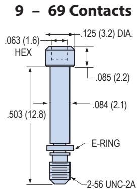
Kit Part Number 500-080-2 Kit Consists of 2 Jackscrews and 2 E-Rings
