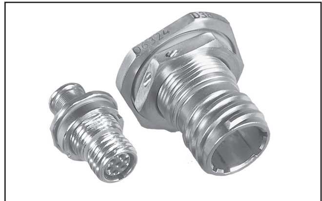
The 7-pin Glenair Series 80 "Mighty Mouse" Connector (left) serves reliably in missile systems, satellites, geophysical exploration and on the battlefield. The equivalent D38999 Connector (right) is nearly twice the size and weight.
